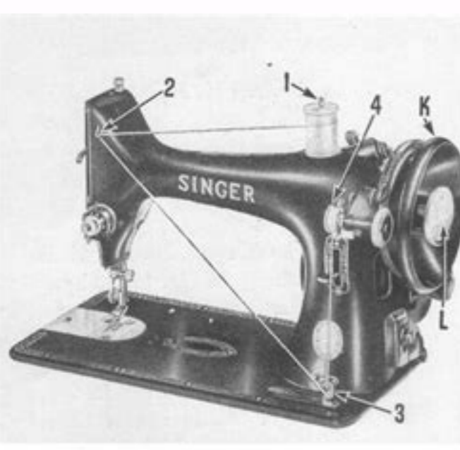
Fig. 11. Machine Threaded for Winding the Bobbin
