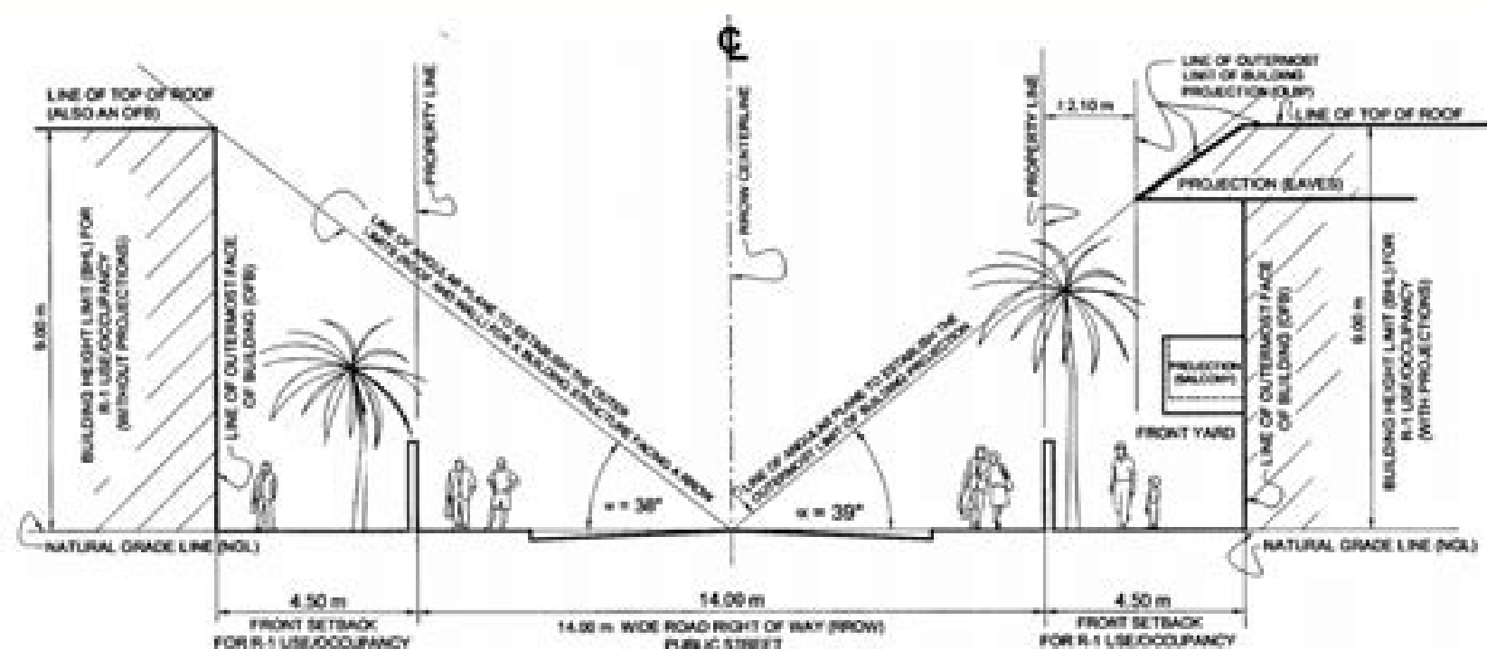
ANGLES FROM CENTERLINE THAT DETERMINE THE OFB AND OLB OF R-1 BUILDINGS/STRUCTURES (WITH AND WITHOUT PROJECTIONS) ALONG A 14.00 M RROW
